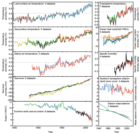
IPCC 2013 figure TS.01
